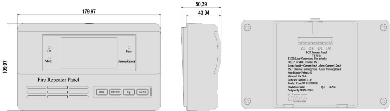
Fig.1 LCD Repeater Panel Structure
