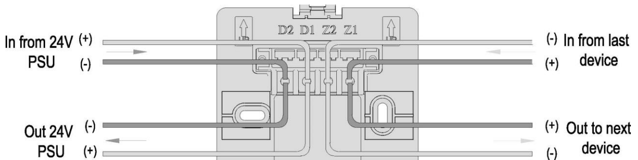
Fig.1 LCD Repeater Panel Structure
